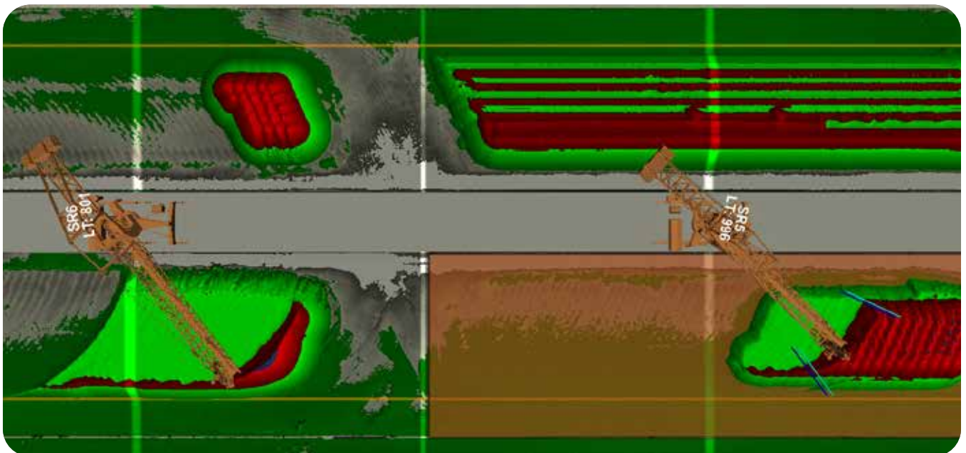
Highly accurate 3D visualisation with the colours showing bench heights and a mix of stacking methods including windrow and cone slew.
