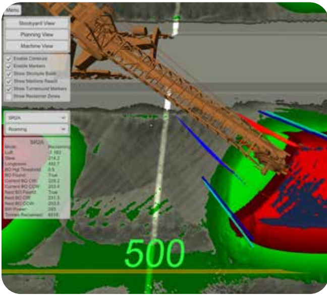
Machine metrics and laser data points are used to calculate turnaround slew position for the current and next slew swings.
